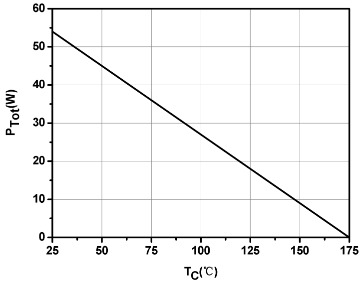
Fig.5-Power Derating
